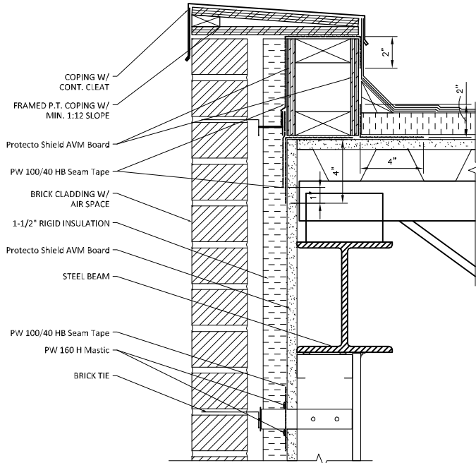
Roofing / Parapet Interface
