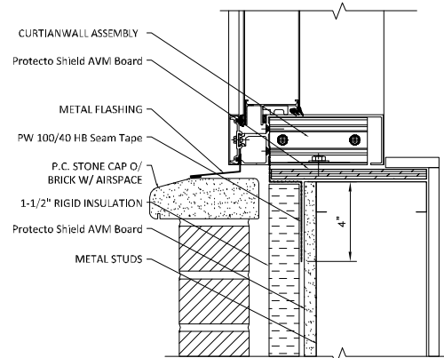
Window Sill
