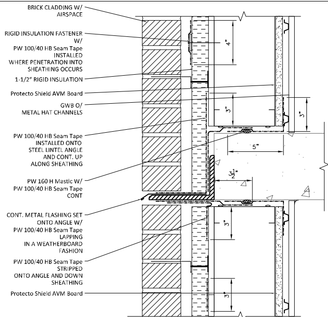
Shelf Angle A
