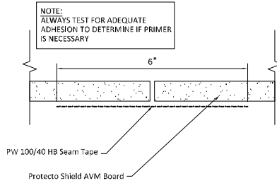
Typical Joint
