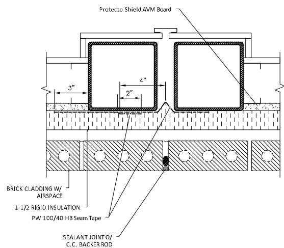
Expansion Joint
