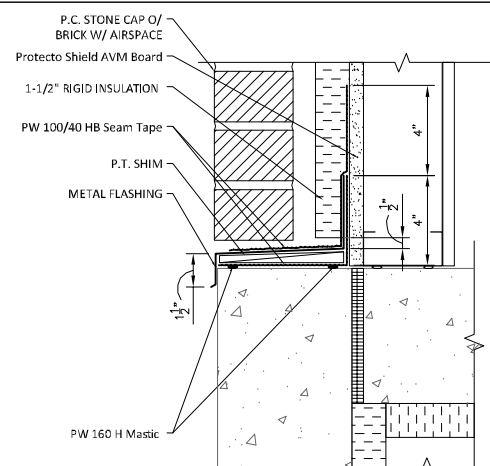
Foundation Interface A
